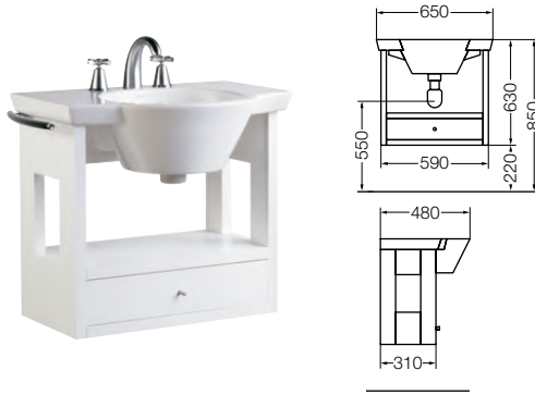
Conjunto lavatorio 65 cm y mueble colgante Set lavatory 65 cm and hanging furniture YH61C BB / EB / SB (1 agujero) / (1 hole) YH63C BB / EB / SB (3 agujeros) / (3 holes)
