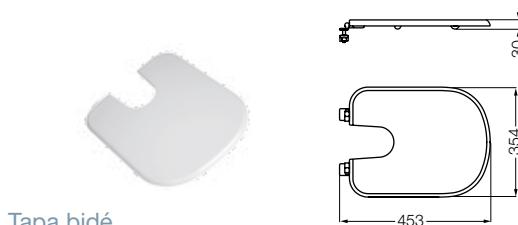
Tapa bidé Cover seat for bidet TBKP B (1 agujero) / (1 hole) - herraje plástico plastic ironwork (MDF)
