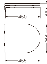
Tapa y asiento inodoro Toilet seat and cover TRXUS B - cierre suave /soft close (UF) TRIM B - herraje metálico / metallic ironwork (MDF)
