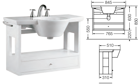
Conjunto lavatorio 85 cm y mueble colgante Set lavatory 85 cm and hanging furniture YH81C BB / EB / SB (1 agujero) / (1 hole) YH83C BB / EB / SB (3 agujeros) / (3 holes)
