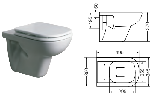
Inodoro de colgar Toilet to be hung up IKPJ B
